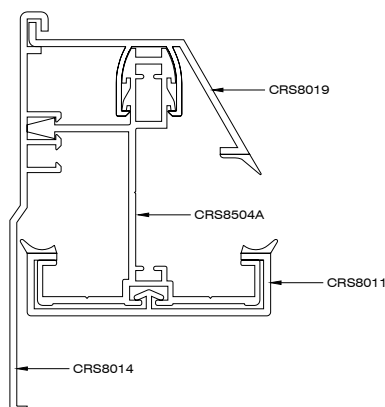
GABLE RAFTER ASSEMBLY
