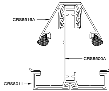
LIGHTWEIGHT RAFTER ASSEMBLY
